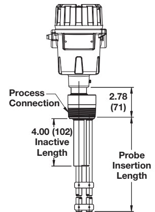
Model 7XB Twin Rod Probe NPT Threaded Connection
