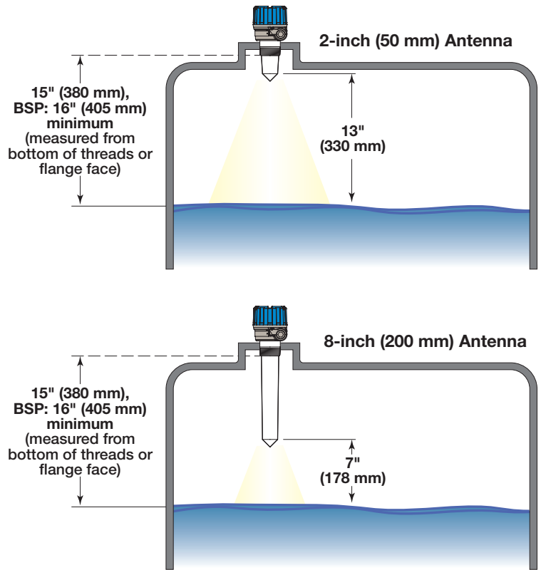
Figure 6 Minimum Blocking Distance
