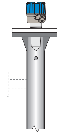
Figure 10 Use in Standpipe/Stillwell
