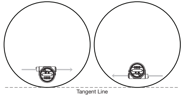
Figure 9 Launcher Orientation
