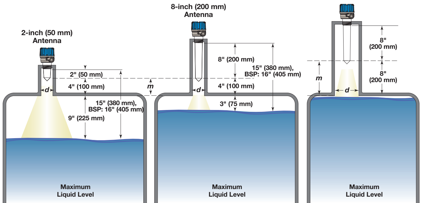
Figure 7 Maximizing Useable Capacity
