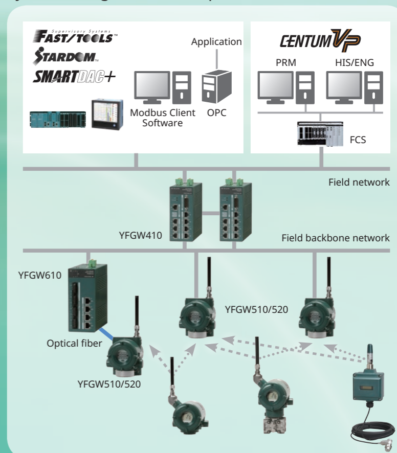
System configuration example #2
